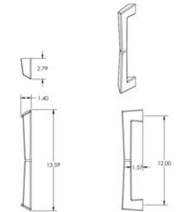
Fold + taper at custom door pulls
