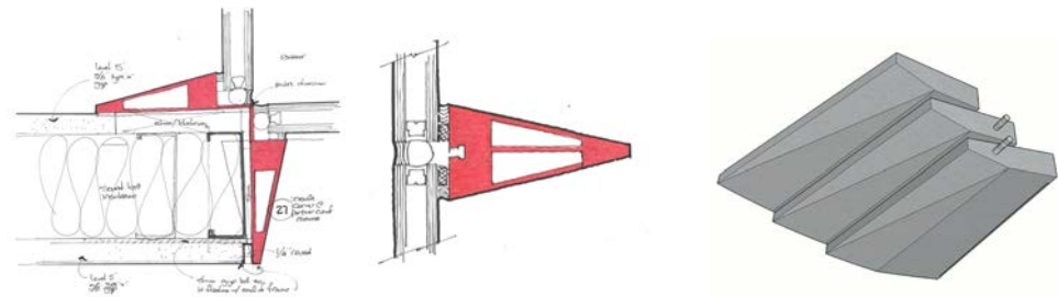
Custom blade mullion profile at exterior + interior windows Fold + taper at underside of concrete stair
